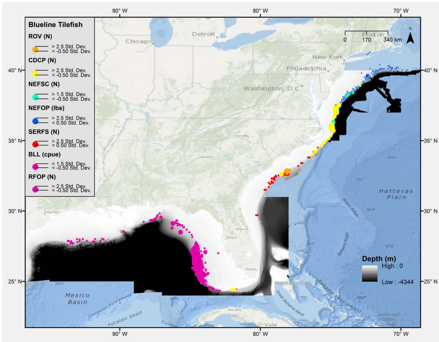
Figure 10. Positive encounters (circles) of blueline tilefish by various sampling programs from the Gulf of Mexico to the Gulf of Maine relative to bathymetry from the Coastal Relief Model. NMFS-BLL and RFOP encounters with blueline tilefish are presented under the same color scheme to protect confidentiality.
